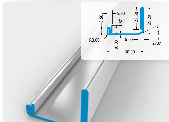
Veka 113.294
