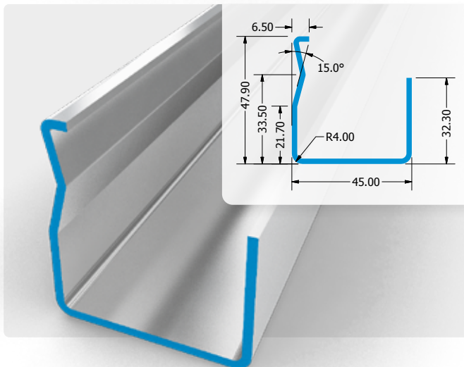
Veka 113.270
