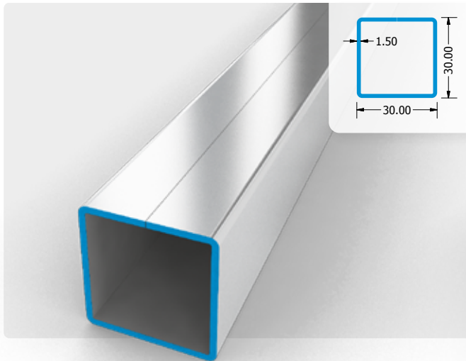
Veka 113.025
